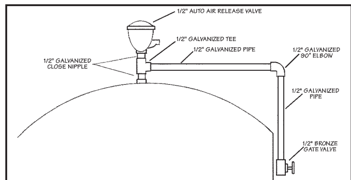
TFB Automatic and Manual Air Release Assembly
